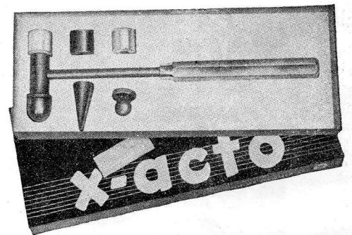
No. 50 X-acto HAMMER SET — Designed for art metal work, model railroad work, etc. Interchangeable-head hammer set with 6 different heads: 2 steel ball, 1 flat steel, 1 flat brass, 1 flat plastic, 1 tinner's steel. Tinner's head has set screw for locking striking edge at any angle. All metal handle 7" long. Boxed complete $1.50
