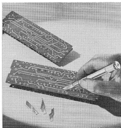
CORRECTING PRINTED CIRCUIT BOARDS.
