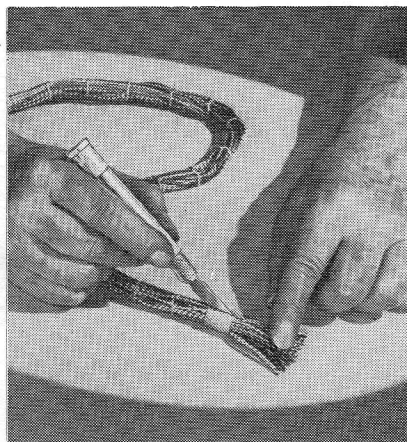
CUTTING HARNESS LACING ON WIRES.
