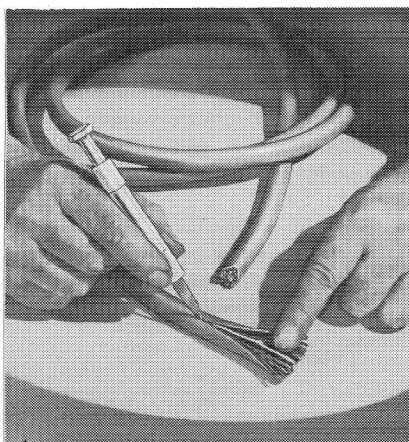
STRIPPING INSULATION FROM CABLE.
